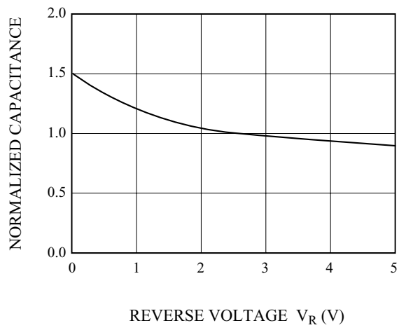
C_J - V_R
