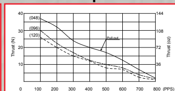
Bipolar Constant Voltage 48x4 Torque Curve
