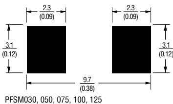
Recommended Pad Layout
