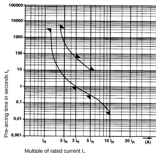
Thermal characteristics without current
