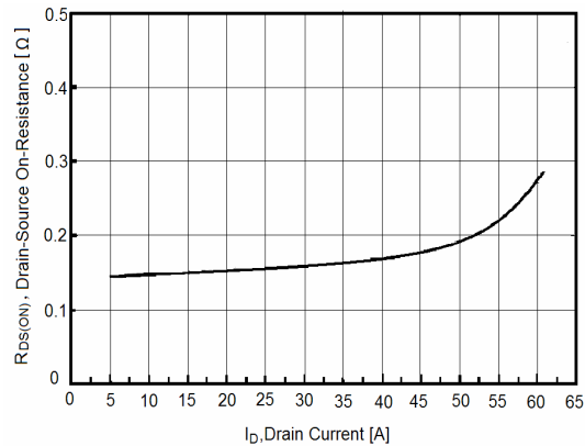
Figure 5. Static Drain-Source On Resistance
