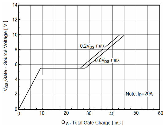
Figure 9. Gate Charge Waveforms
