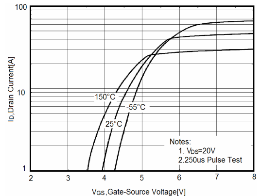
Figure 4. Transfer Characteristics
