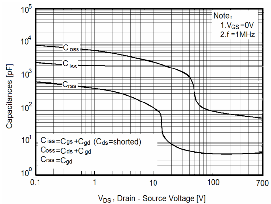
Figure 10. Capacitance
