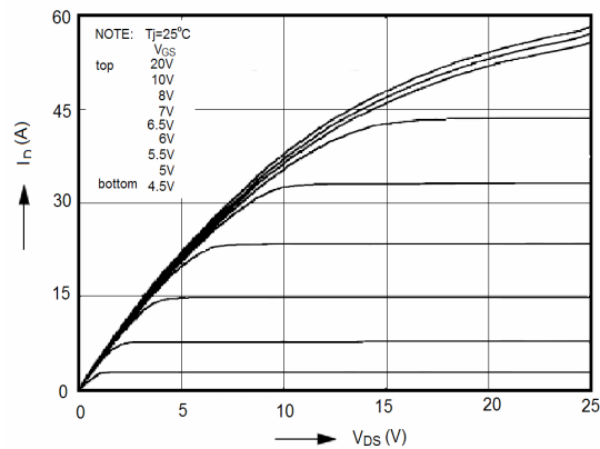
Figure 3. Output Characteristics
