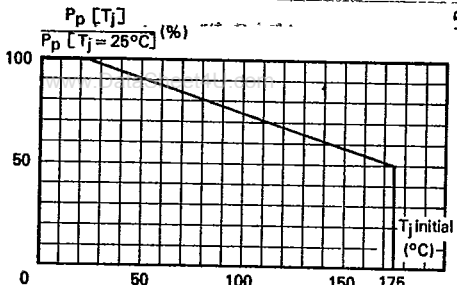
Fig. 4 — Allowable power dissipation versus junction temperature.
