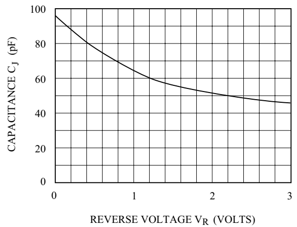
C_J - V_R
