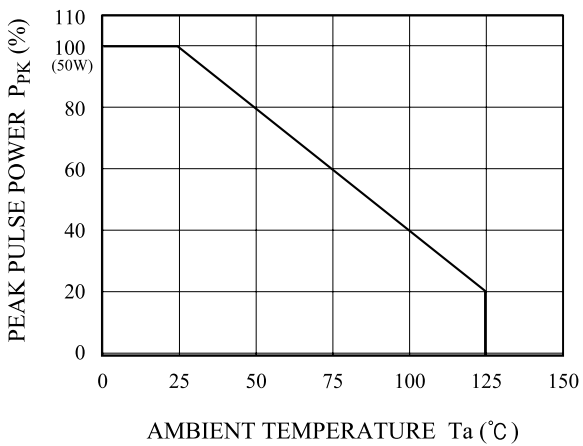
POWR DERATING CURVE
