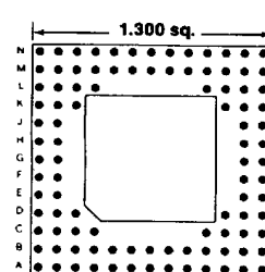
100 PINS
