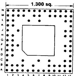
88 PINS Footprint 13049
