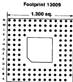
122 PINS
