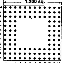
108 PINS Footprint 12005
