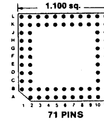
Footprint 11027
