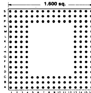
176 PINS Footprint 16007
