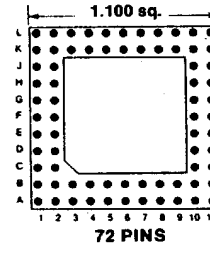
Footprint 11023
