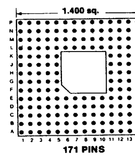
Footprint 14007
