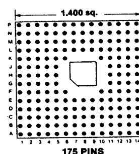
Footprint 14004
