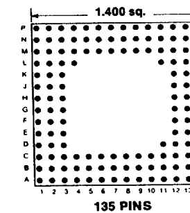
Footprint 14012
