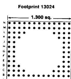
100 PINS
