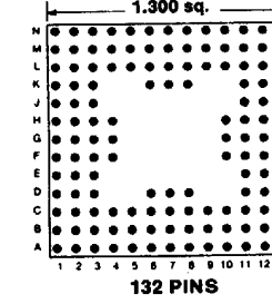
Footprint 13007
