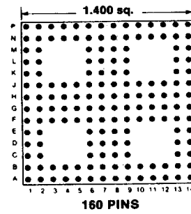
Footprint 14009
