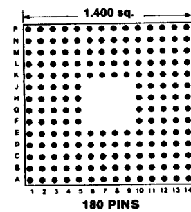
Footprint 14003
