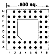
44 PINS Footprint 08002
