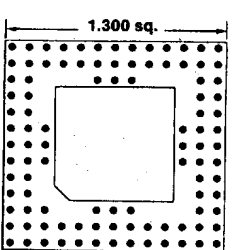
101 PINS
