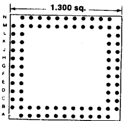
84 PINS Footprint 13053
