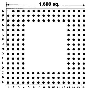
175 PINS Footprint 16003
