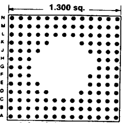
133 PINS Footprint 13054
