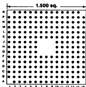
212 PINS Footprint 15004
