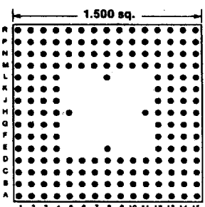
180 PINS Footprint 15008
