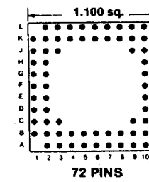
Footprint 11025
