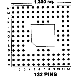
Footprint 13006
