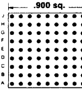
81 PINS Footprint 09001
