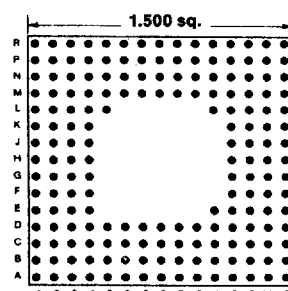
179 PINS Footprint 15012
