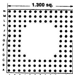
124 PINS
