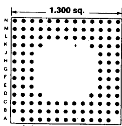
122 PINS
