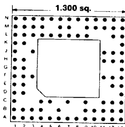
95 PINS Footprint 13047
