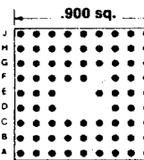
75 PINS Footprint 09002
