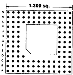
121 PINS
