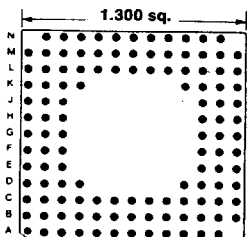
121 PINS Footprint 13058
