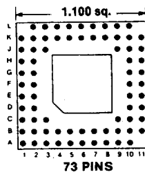
Footprint 11021
