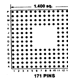
Footprint 14008
