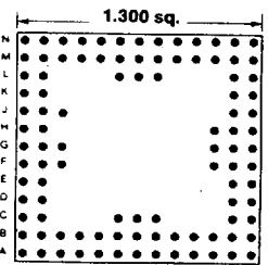
100 PINS Footprint 13059
