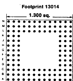
120 PINS
