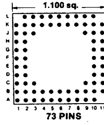
Footprint 11022
