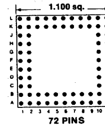
Footprint 11024
