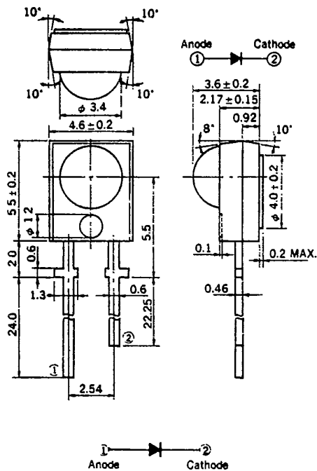
PACKAGE DIMENSIONS in millimeters
