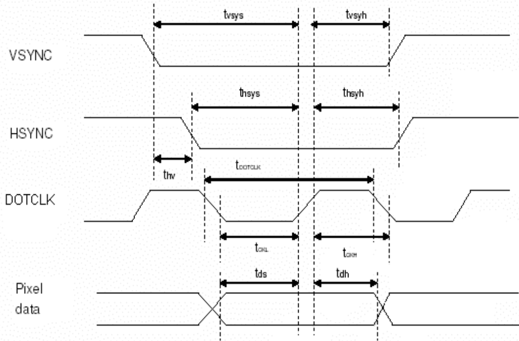
Pixel timing
