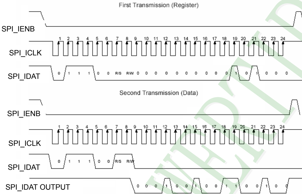
SPI interface Timing Diagram & Read SPI Example
