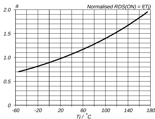
Fig. 9. Normalised drain-source on-state resistance. a = R_{DS(ON)}/R_{DS(ON)25 \text{ °C}} = f(T_J) ; I_D = 10 \text{ A} ; V_{GS} = 10 \text{ V}
