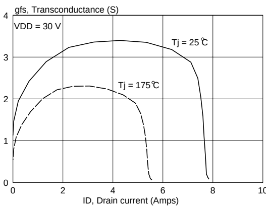
Fig. 8. Typical transconductance. g_{fs} = f(I_D) ; parameter T_J
