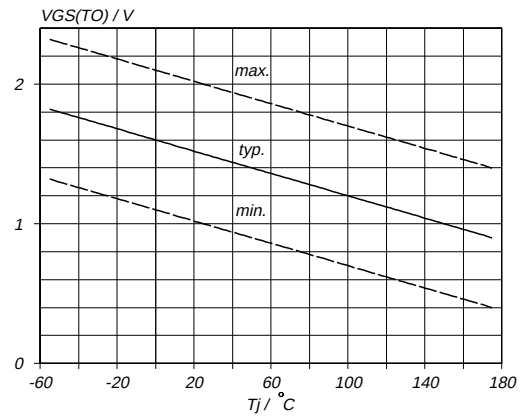
Fig. 10. Gate threshold voltage. V_{GS(T0)} = f(T_J) ; conditions: I_D = 0.25\text{ mA} ; V_{DS} = V_{GS}
