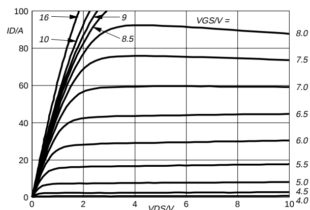
Fig.5. Typical output characteristics, T_j = 25\ ^\circ C . I_D = f(V_{DS}) ; parameter V_{GS}
