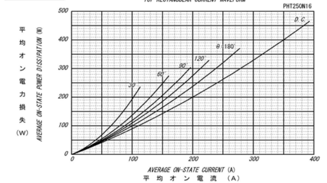
平均オン電力損失特性 AVERAGE ON-STATE POWER DISSIPATION for RECTANGULAR CURRENT WAVEFORM
