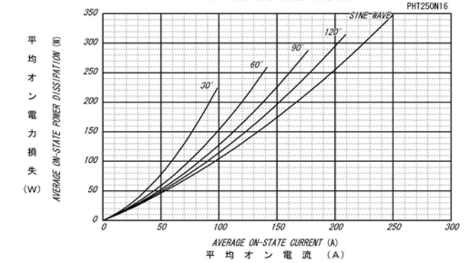
平均オン電力損失特性 AVERAGE ON-STATE POWER DISSIPATION for SINUSOIDAL CURRENT WAVEFORM
