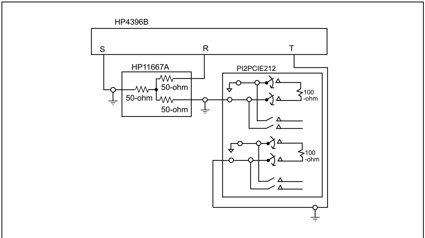
Fig 1. Crosstalk Setup
