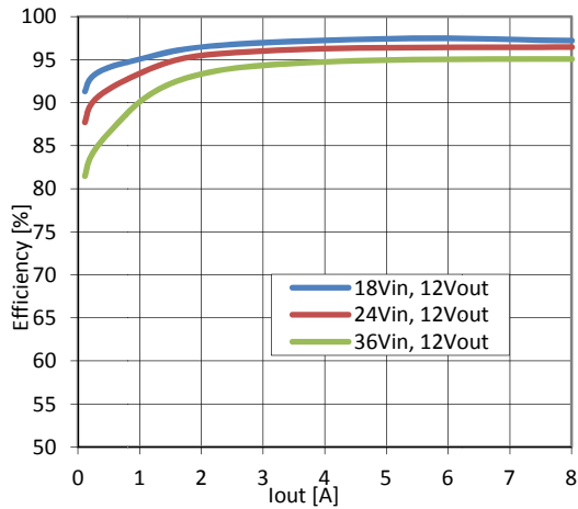
Efficiency at 25°
