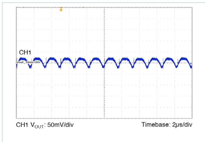
Figure 26 — Output Ripple 24VIN, 3.3VOUT at 10A
