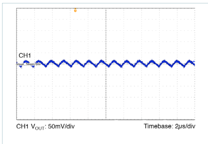
Figure 27 — Output Ripple 24VIN, 3.3VOUT at 5A
