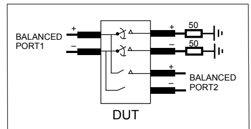
Fig 3: Diff. Off Isolation Test Circuit
