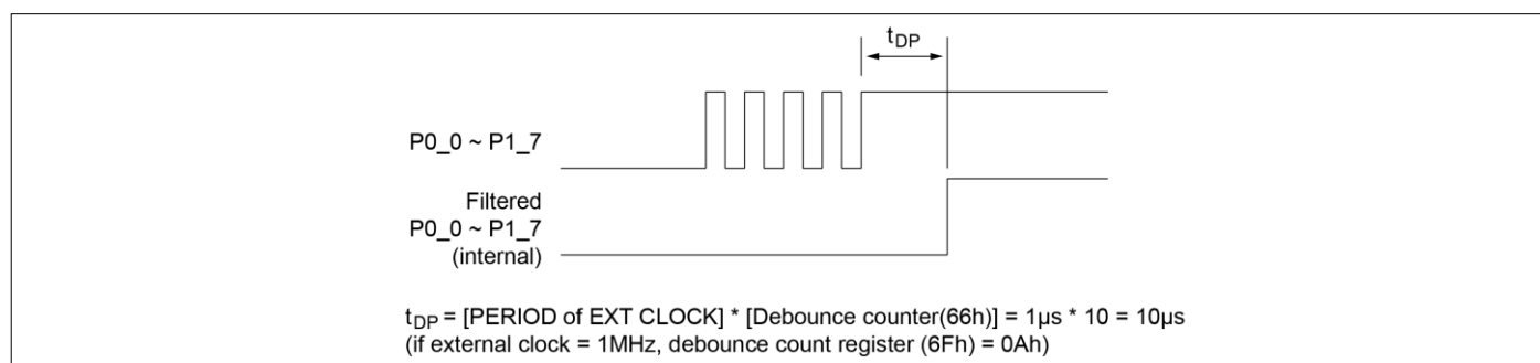
Figure 13. Switch Debounce Timing
