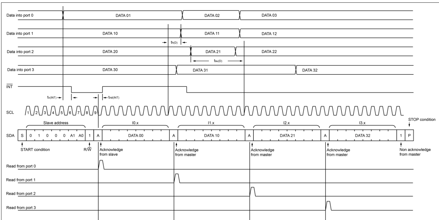
Figure 5. Read Input Port Register (non-latched), Scenario 2
