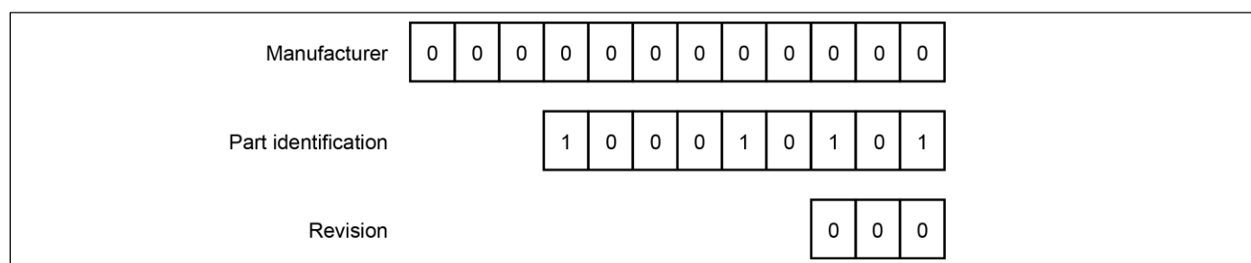
Figure 8. PI4IOE5V6534Q Device ID Field
