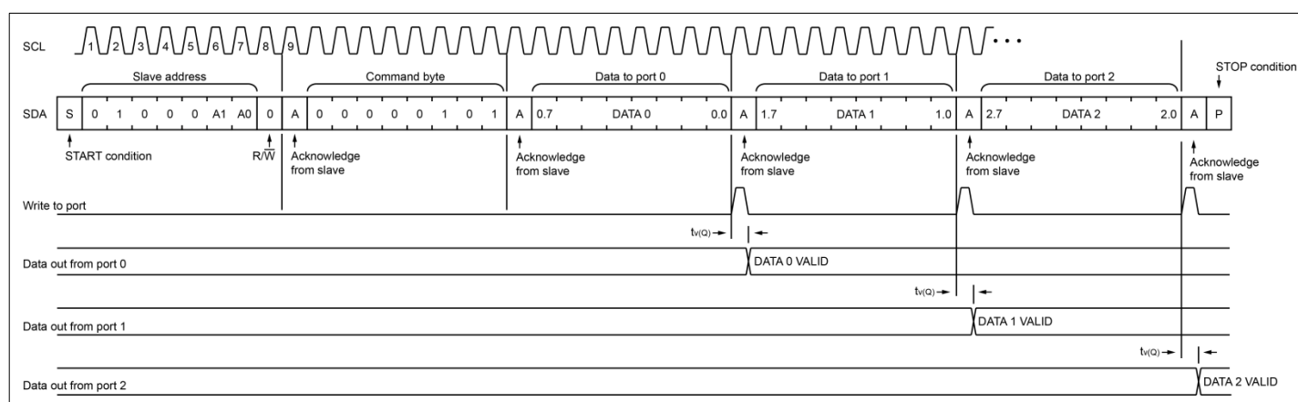
Figure 1. Write to Output Port Register
