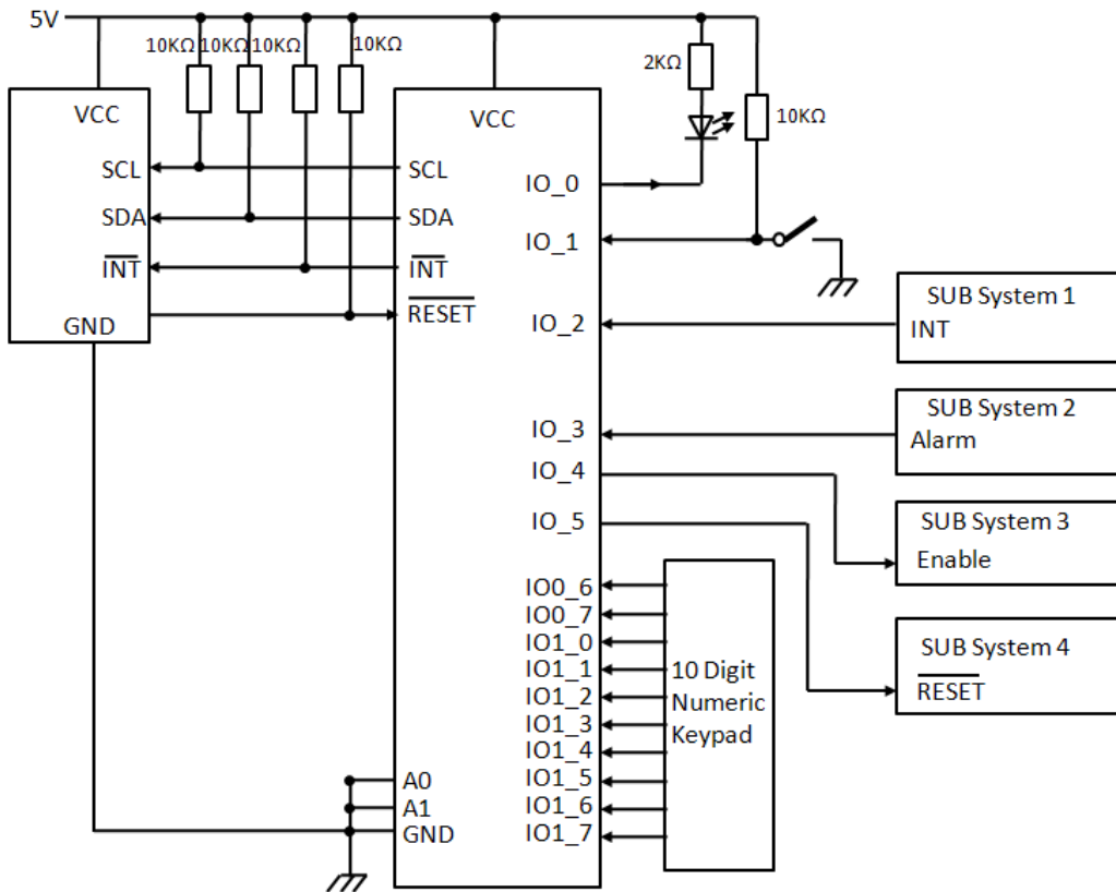
Figure 10: Typical application
