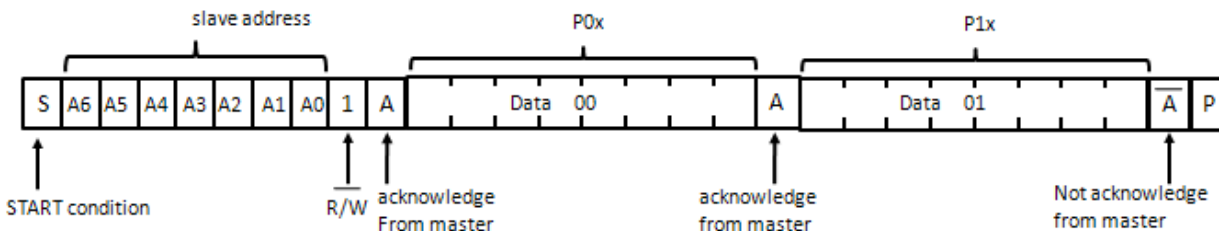
Figure 9. Read input port register
