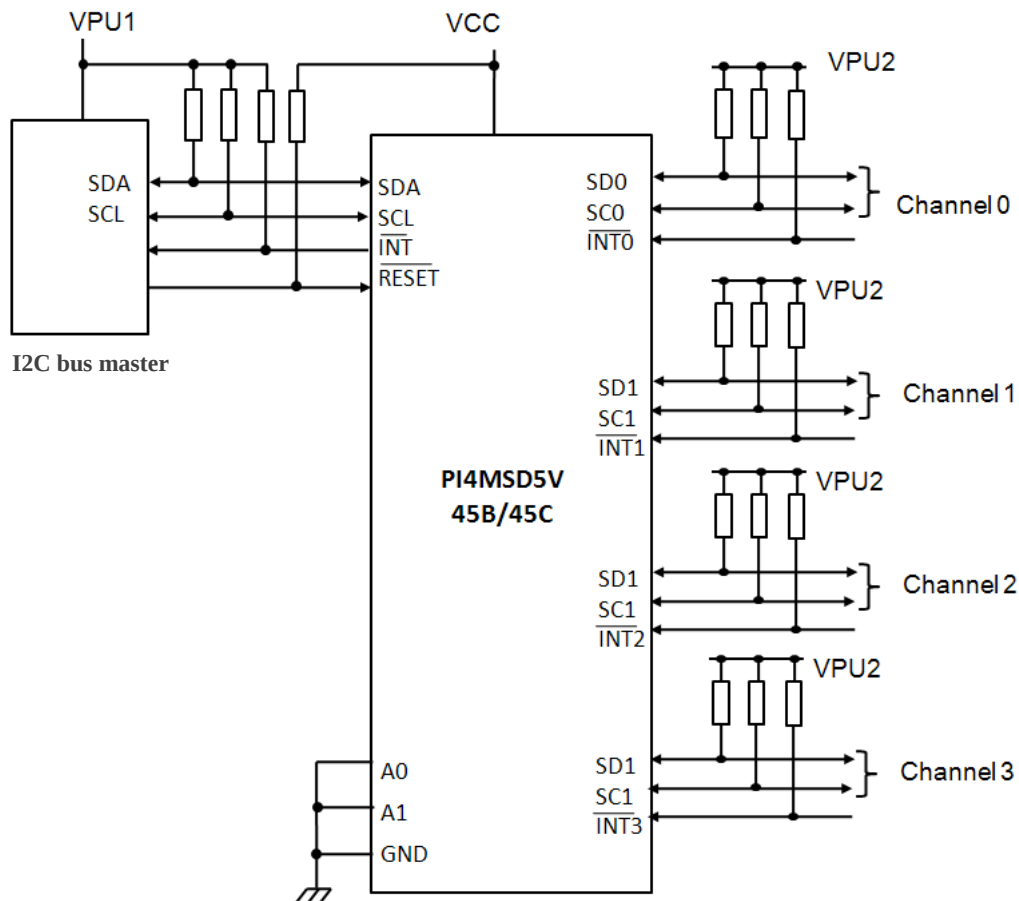
Figure 3. Typical Application
