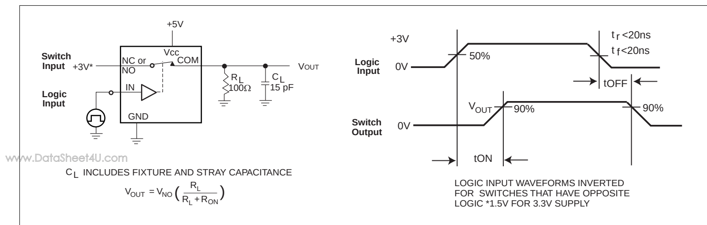
Figure 1. Switching Time
