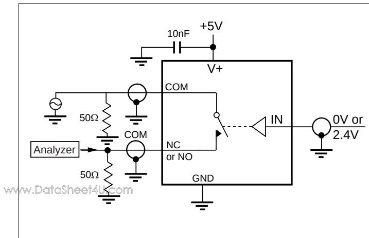
Figure 3. Off Isolation
