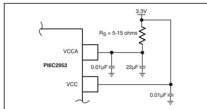
Figure 6. Power Supply Filter www.DataSheet4U.com
