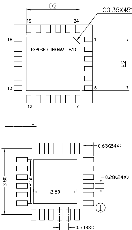
RECOMMENDED LAND PATTERN (TOP VIEW)
