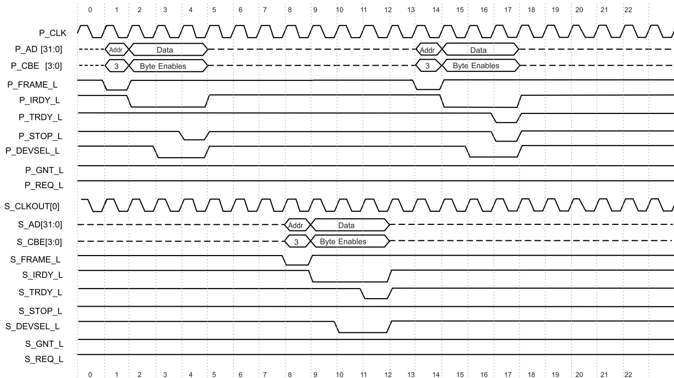
Figure 27. Downstream Delayed I/O Write Transaction ( P --> S )
