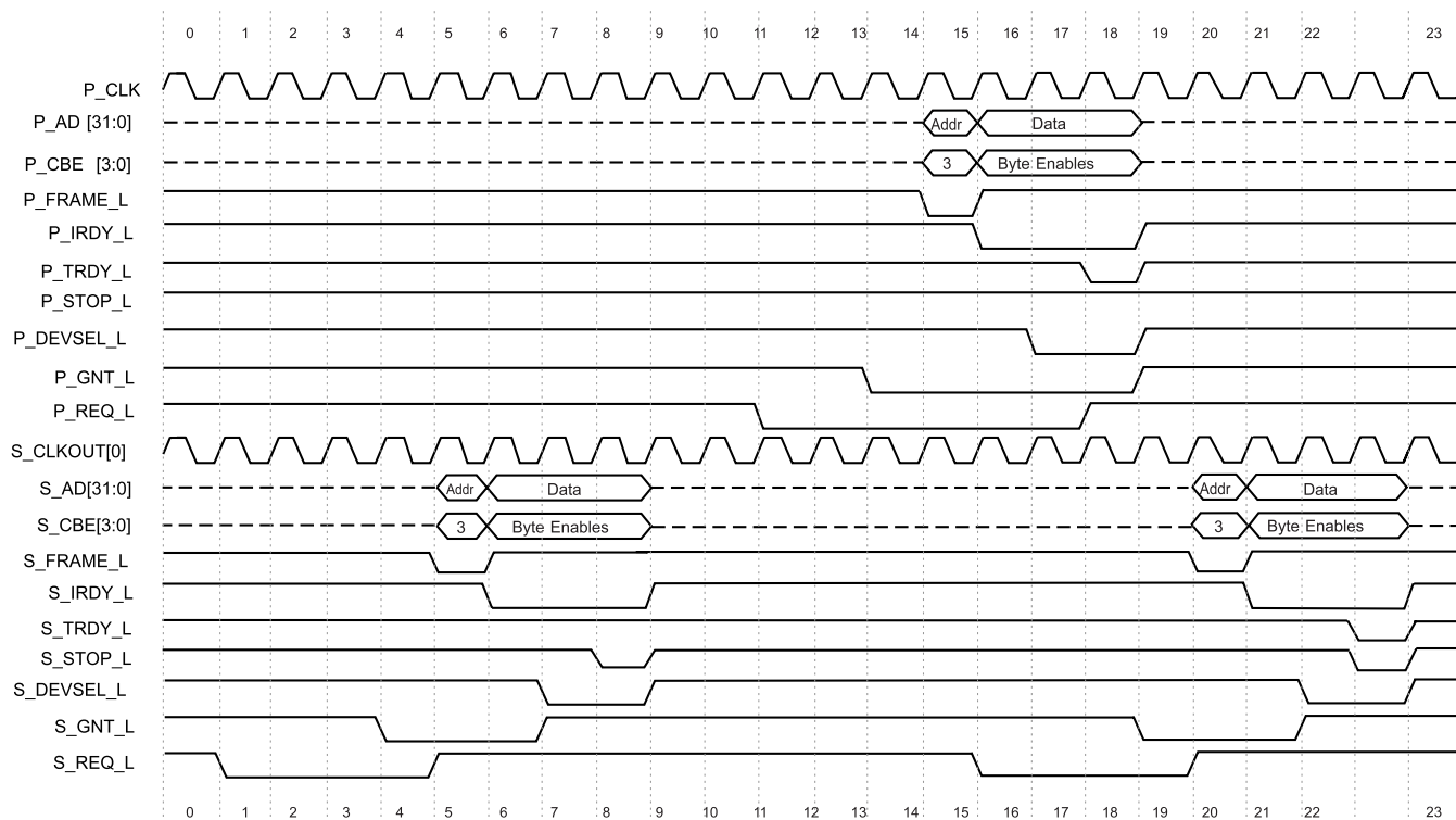
Figure 30. Upstream Delayed I/O Write Transaction ( S --> P )
