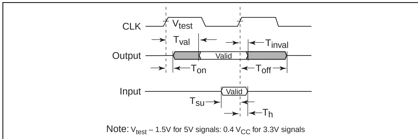
Figure 16-1. PCI Signal Timing Measurement Conditions
