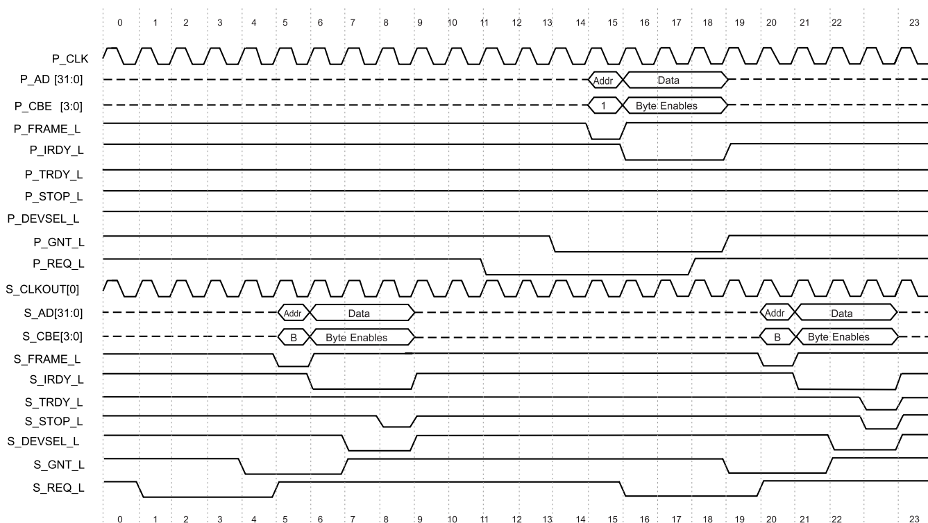
Figure 5. Upstream Type 1 to Special Cycle Transaction ( S --> P )
