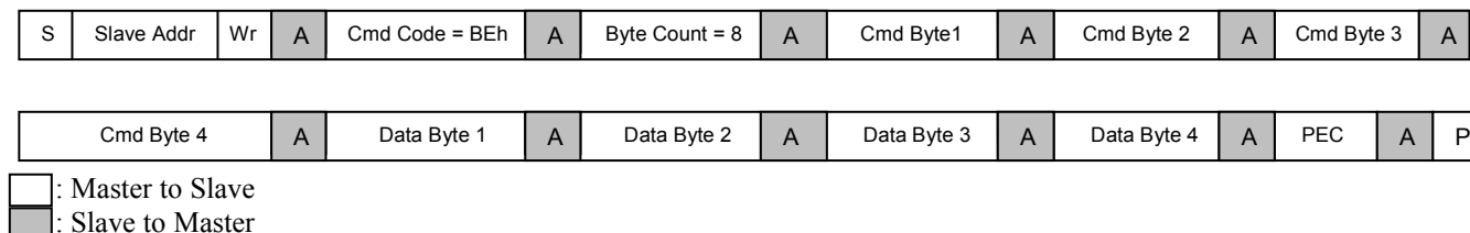
Figure 7-3 SMBus Block Write Command Format, to Write to a PI7C9X2G808PR Register with PEC
