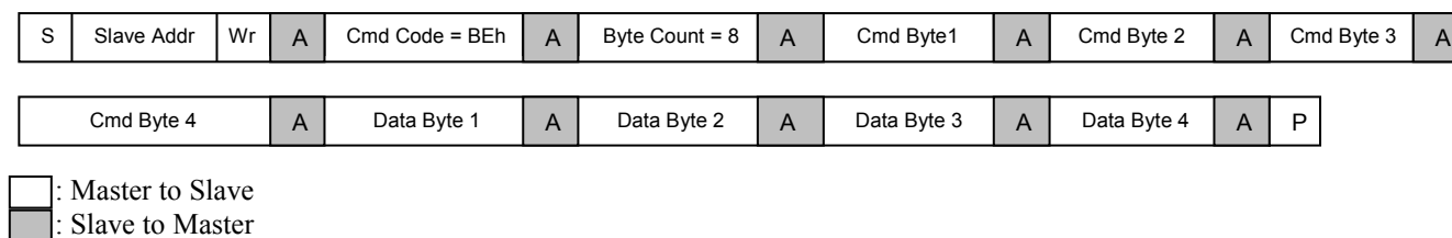
Figure 7-2 SMBus Block Write Command Format, to Write to a PI7C9X2G808PR Register without PEC
