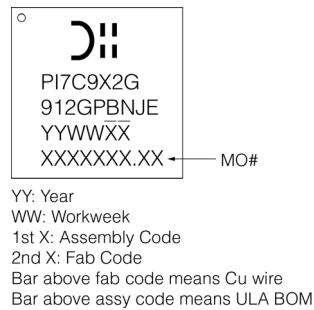
Figure 15-2 Part Marking
