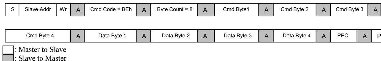
Figure 7-3 SMBus Block Write Command Format, to Write to a PI7C9X2G912GP Register with PEC
