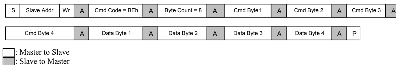
Figure 7-2 SMBus Block Write Command Format, to Write to a PI7C9X2G912GP Register without PEC
