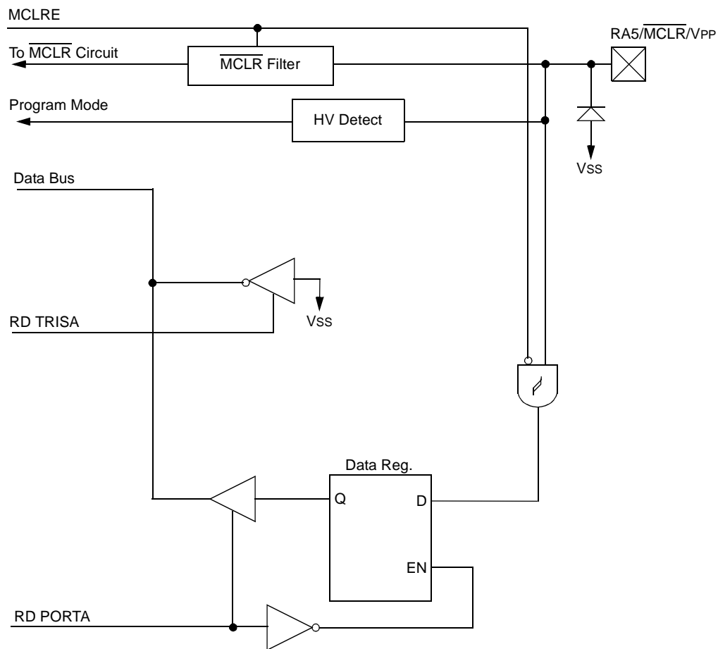
FIGURE 3-6: BLOCK DIAGRAM OF RA5/MCLR/VPP PIN
