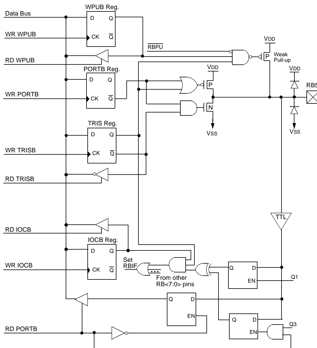
FIGURE 3-14: BLOCK DIAGRAM OF RB5 PIN
