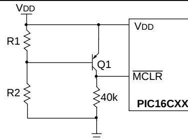
FIGURE 8-15: BROWN-OUT PROTECTION CIRCUIT 2
