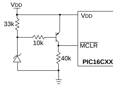
FIGURE 8-14: BROWN-OUT PROTECTION CIRCUIT 1
