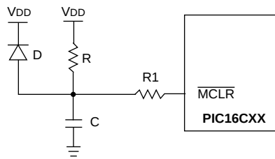
FIGURE 8-13: EXTERNAL POWER-ON RESET CIRCUIT (FOR SLOW V DD POWER-UP)
