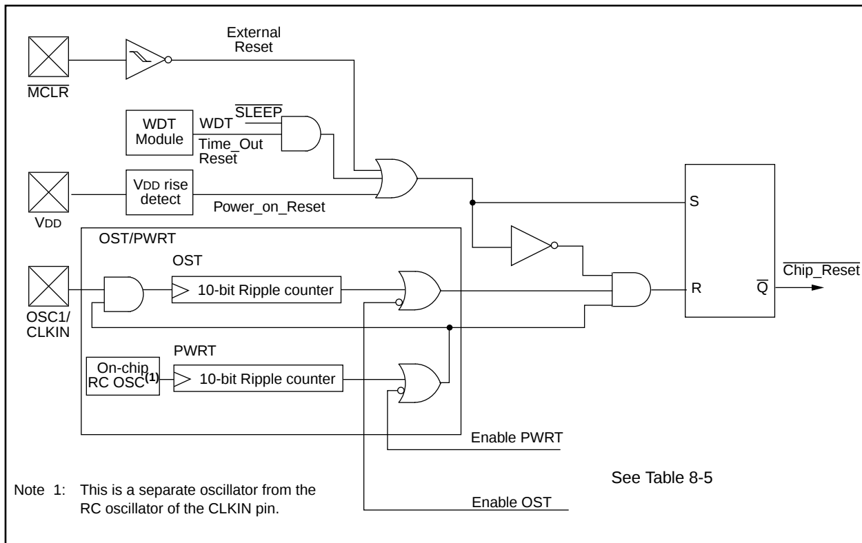
FIGURE 8-9: SIMPLIFIED BLOCK DIAGRAM OF ON-CHIP RESET CIRCUIT
