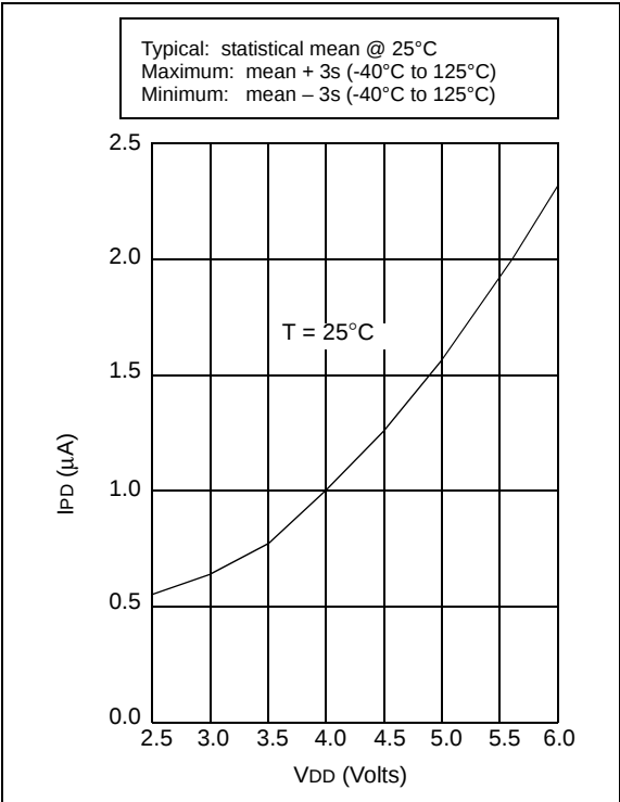
FIGURE 14-5: TYPICAL IPD vs. VDD, WATCHDOG DISABLED
