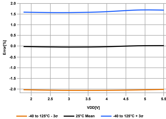
Figure 33-17. HFINTOSC Error % over V_{DD}
