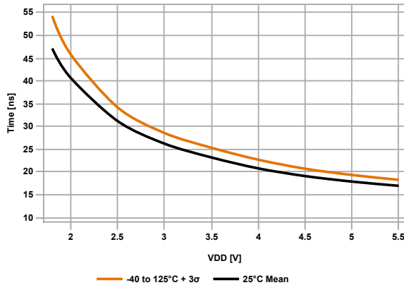
Figure 33-19. Rise Time, Slew Rate Control Enabled
