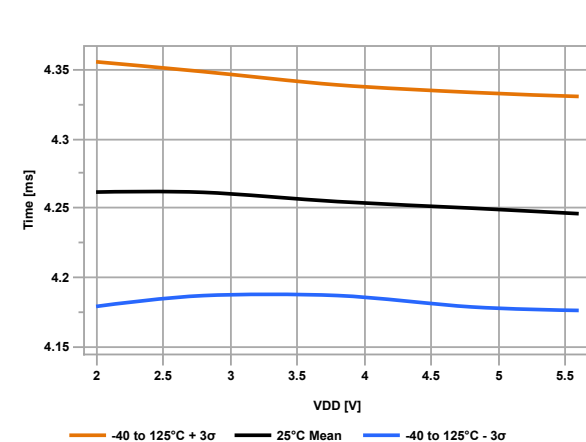
Figure 33-40. WDT Base Time-out Period (WDTPS = 00010 (4 ms))
