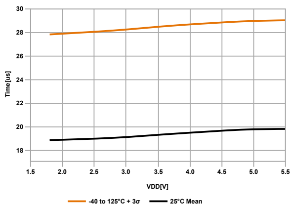
Figure 33-16. Wake from Sleep, HFINTOSC = 4 MHz
