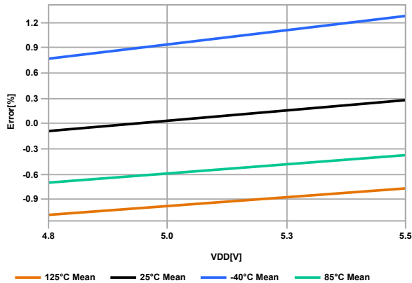
Figure 33-15. FVR Voltage Error 4x ( V_{DD} = 5.5 V)
