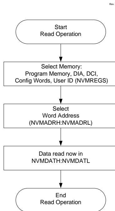
Figure 15-1. Program Flash Memory Read Sequence
