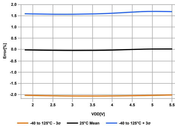
Figure 33-16. HFINTOSC Error % over V_{DD}
