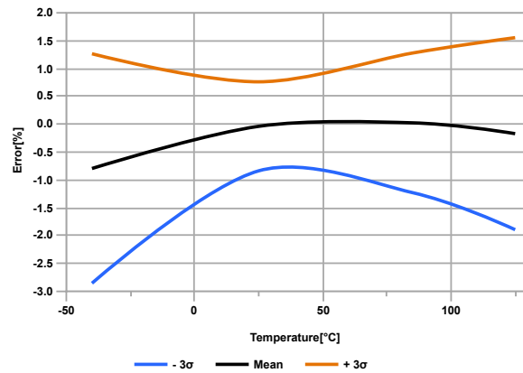
Figure 33-17. HFINTOSC Error % over Temperature, V_{DD} = 3 V
