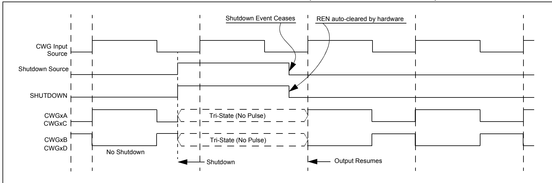
FIGURE 28-14: SHUTDOWN FUNCTIONALITY, AUTO-RESTART ENABLED (REN = 1, LSAC = 01, LSBSD = 01)
