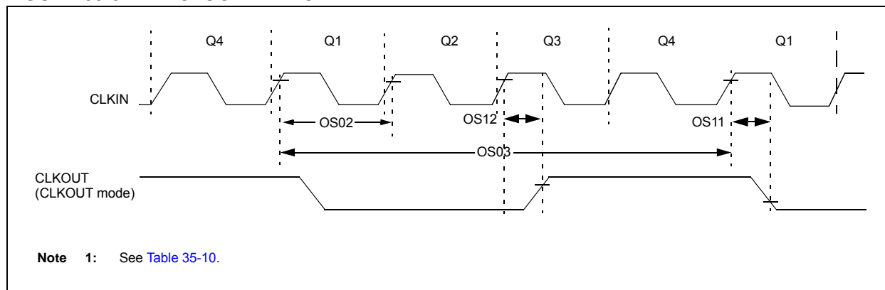
FIGURE 35-5: CLOCK TIMING
