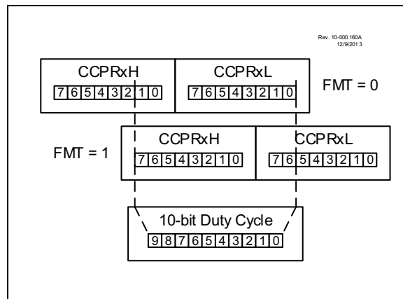
FIGURE 26-4: CCPx DUTY-CYCLE ALIGNMENT
