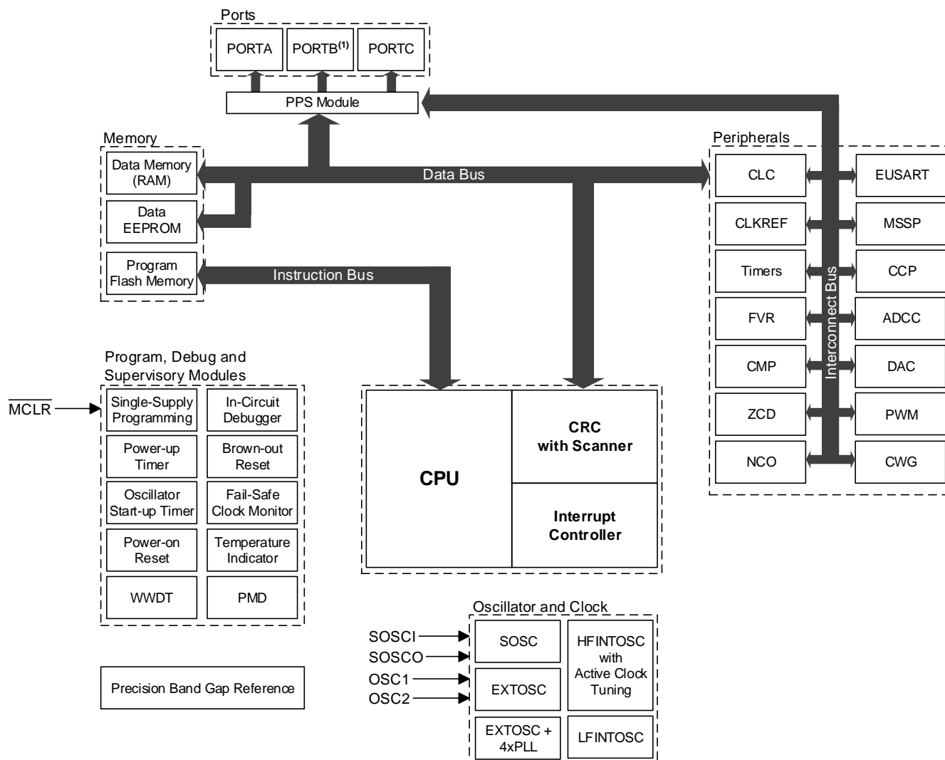
Figure 1. PIC16F18126/46 Block Diagram
