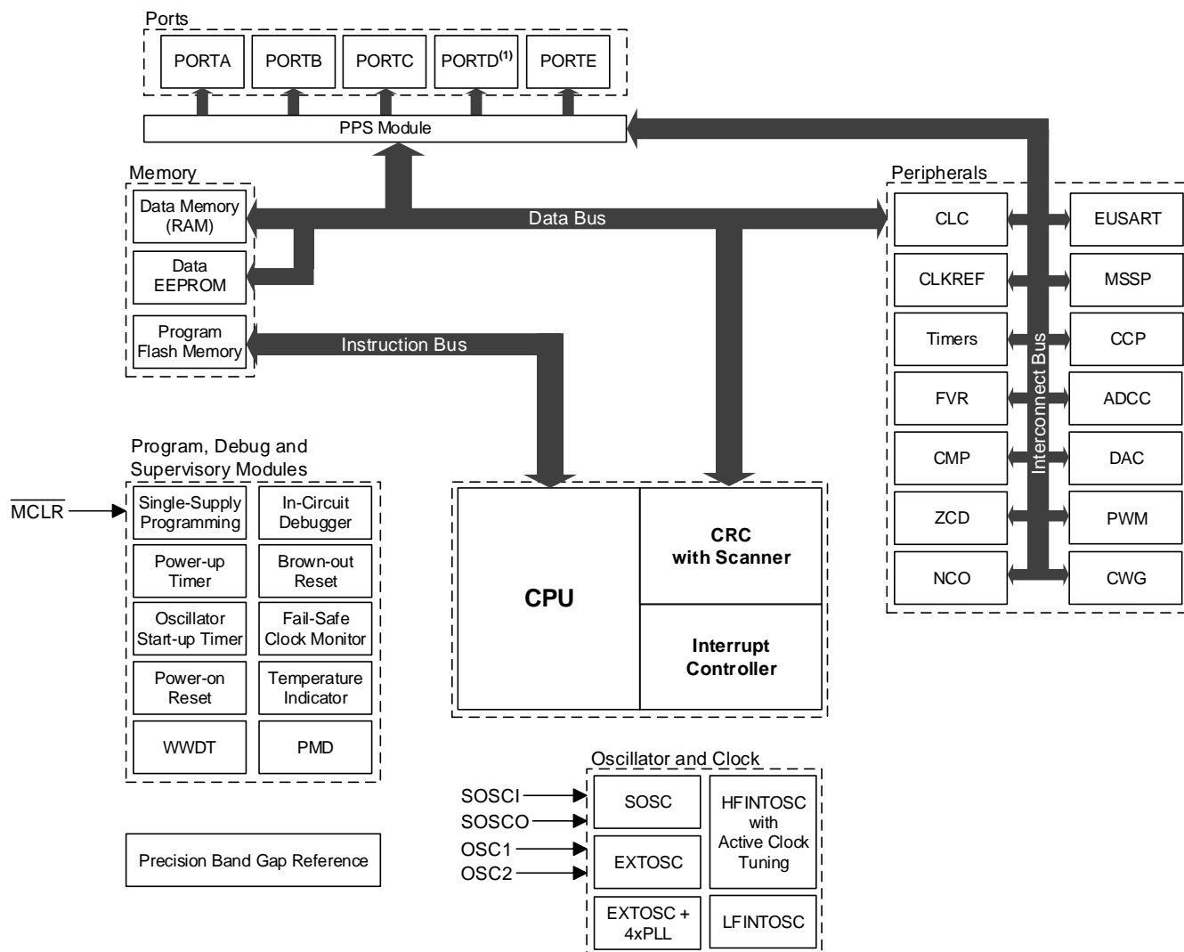
Figure 1. PIC16F18154/55/74/75 Block Diagram
