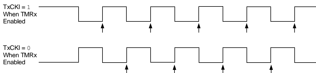
Figure 23-2. Timer1 Incrementing Edge
