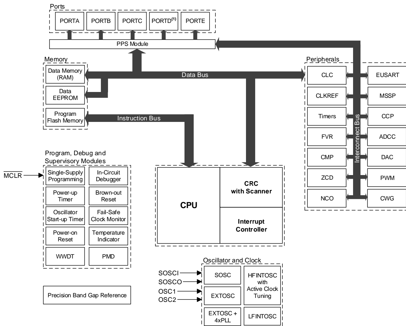
Figure 1. PIC16F18156/76 Block Diagram
