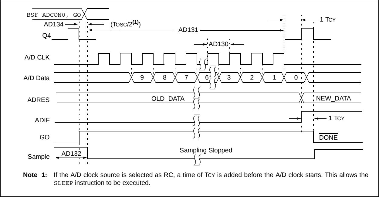
FIGURE 14-10: PIC16F688 A/D CONVERSION TIMING (SLEEP MODE)
