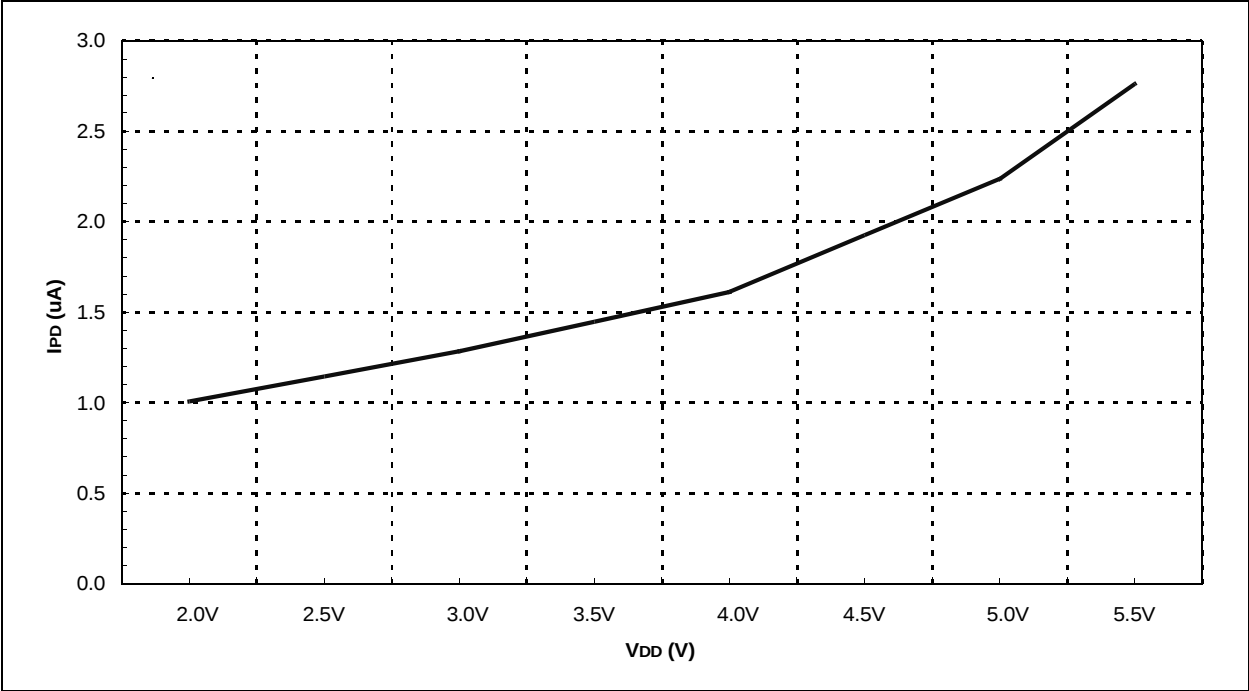
FIGURE 15-17: TYPICAL WDT I PD vs. V DD (25°C)
