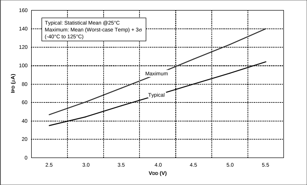
FIGURE 15-16: BOR I PD vs. V DD OVER TEMPERATURE
