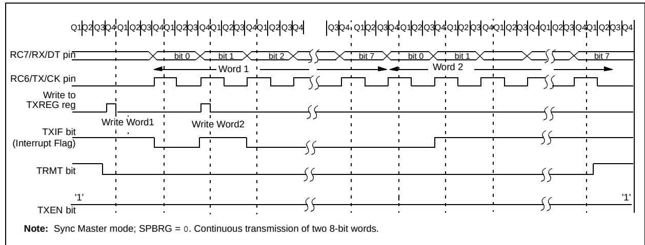
FIGURE 9-9: SYNCHRONOUS TRANSMISSION
