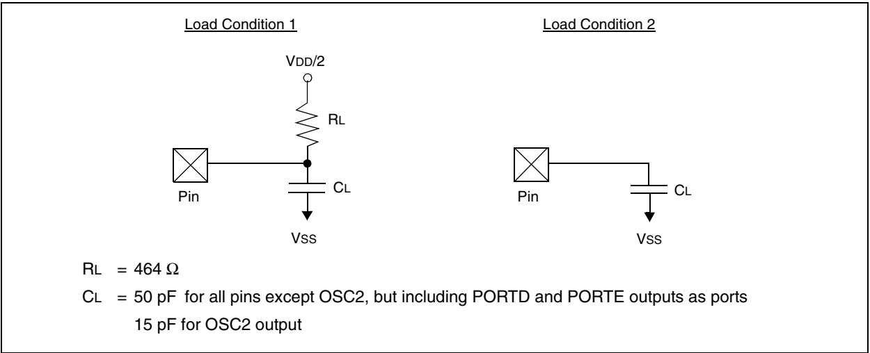
FIGURE 14-3: LOAD CONDITIONS
