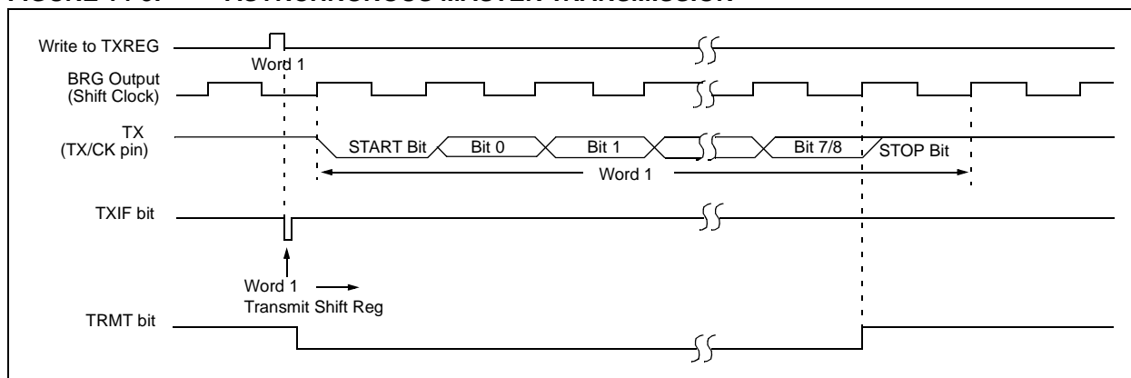
FIGURE 14-3: ASYNCHRONOUS MASTER TRANSMISSION
