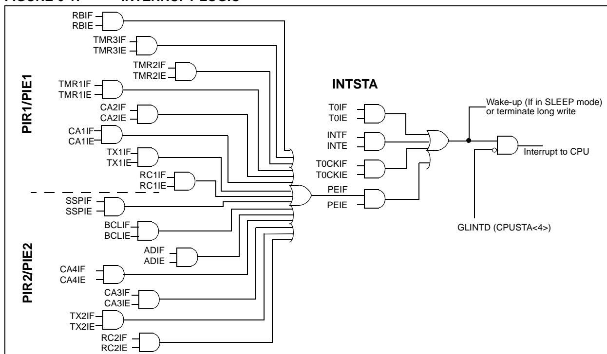
FIGURE 6-1: INTERRUPT LOGIC
