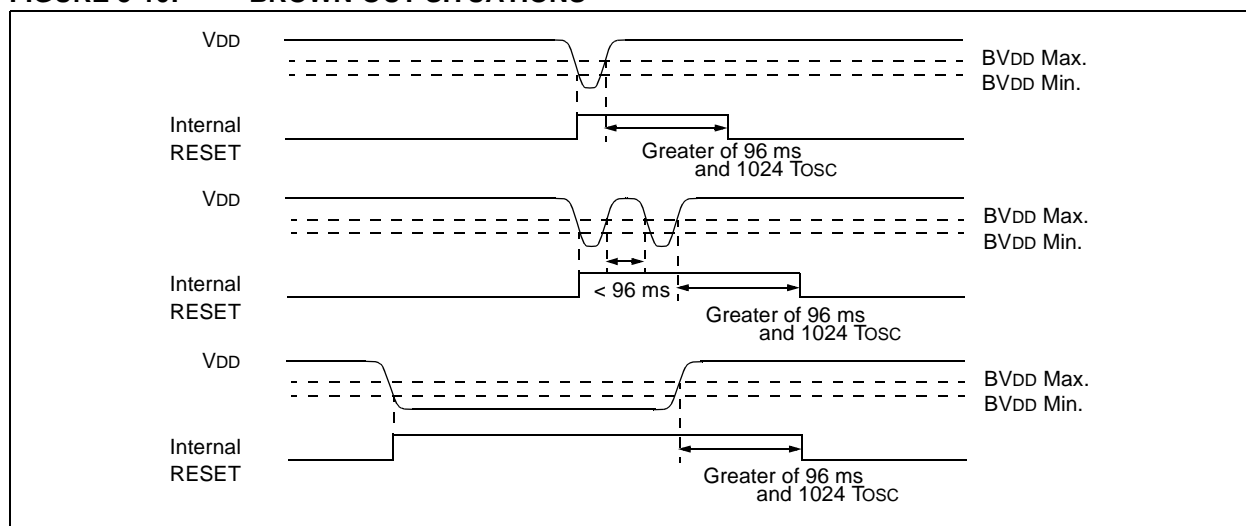
FIGURE 5-10: BROWN-OUT SITUATIONS
