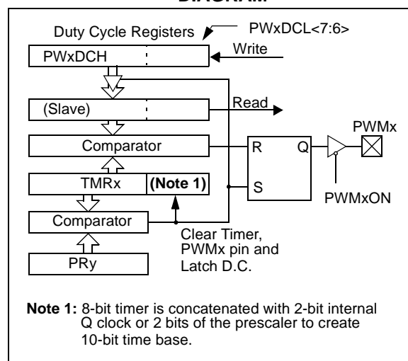
FIGURE 13-3: SIMPLIFIED PWM BLOCK DIAGRAM
