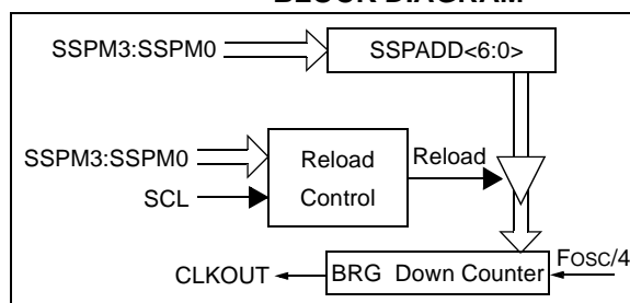
FIGURE 15-18: BAUD RATE GENERATOR BLOCK DIAGRAM
