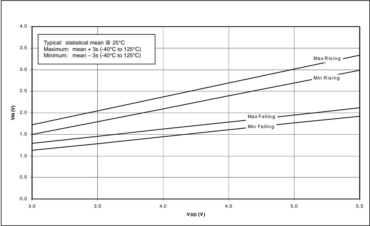
FIGURE 21-23: MAXIMUM AND MINIMUM VIN vs. VDD (I 2 C Input, -40°C to +125°C)
