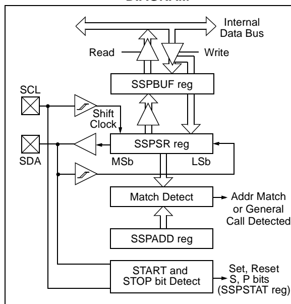
FIGURE 15-2: I 2 C SLAVE MODE BLOCK DIAGRAM
