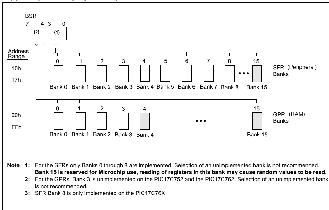
FIGURE 7-9: BSR OPERATION
