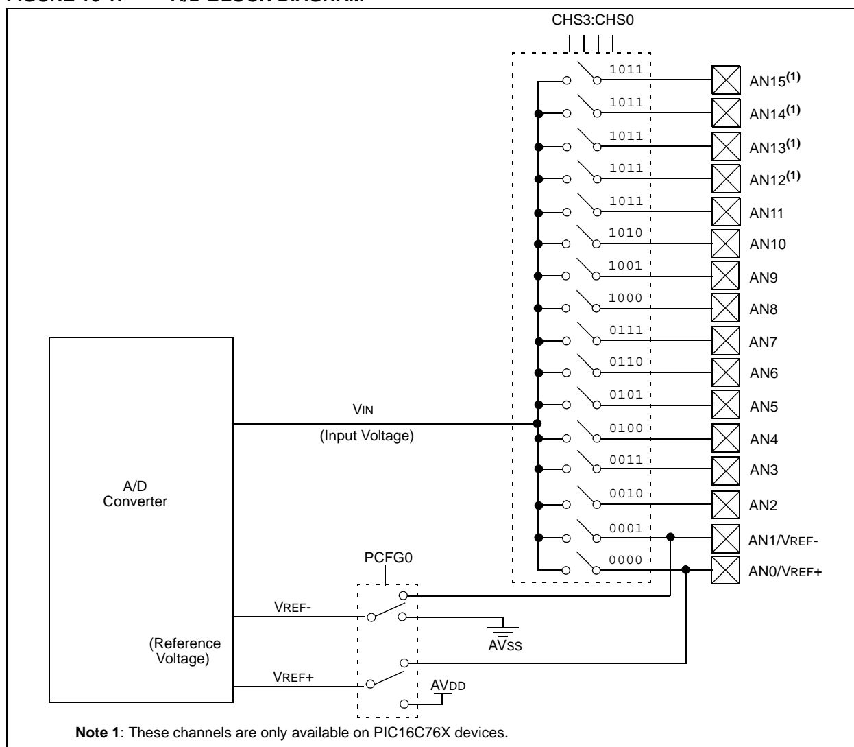
FIGURE 16-1: A/D BLOCK DIAGRAM
