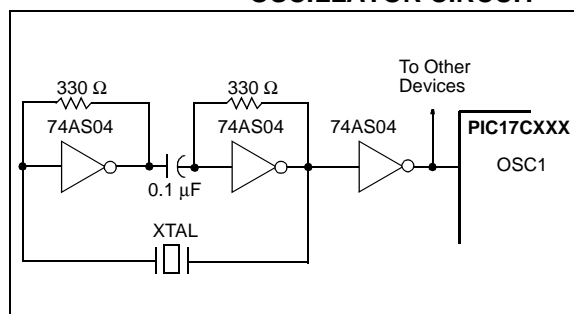
FIGURE 4-6: EXTERNAL SERIES RESONANT CRYSTAL OSCILLATOR CIRCUIT
