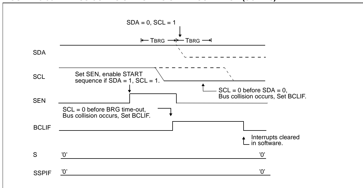
FIGURE 15-36: BUS COLLISION DURING START CONDITION (SCL = 0)
