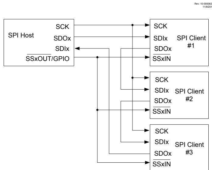
Figure 36-12. Traditional SPI Daisy-Chain Connection
