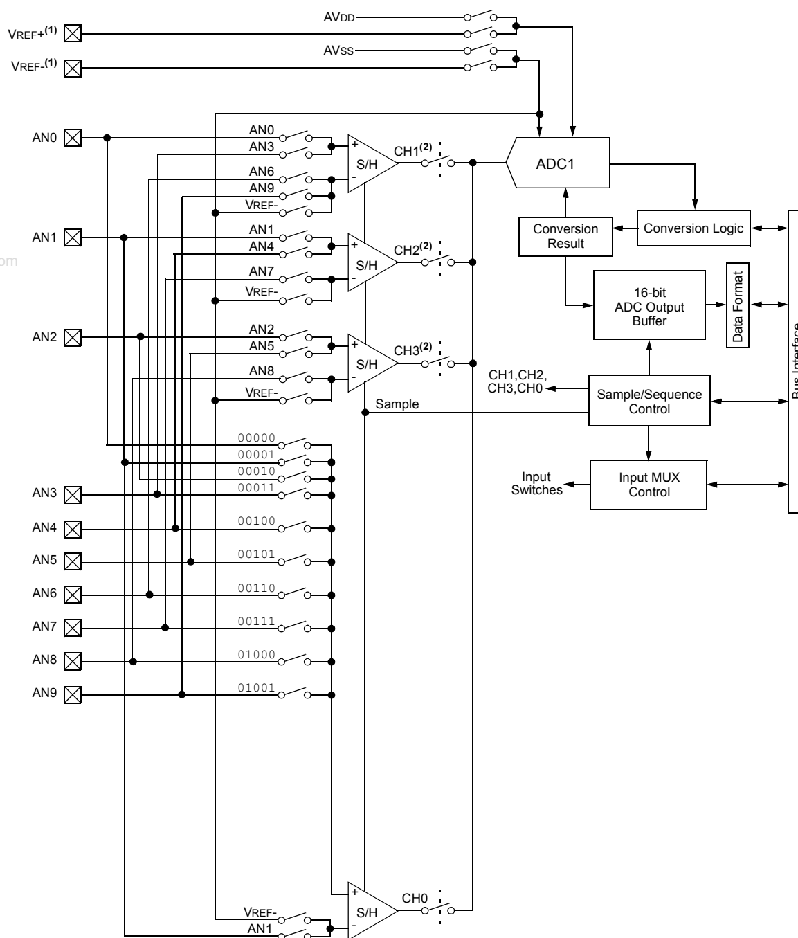
FIGURE 17-1: ADC1 MODULE BLOCK DIAGRAM
