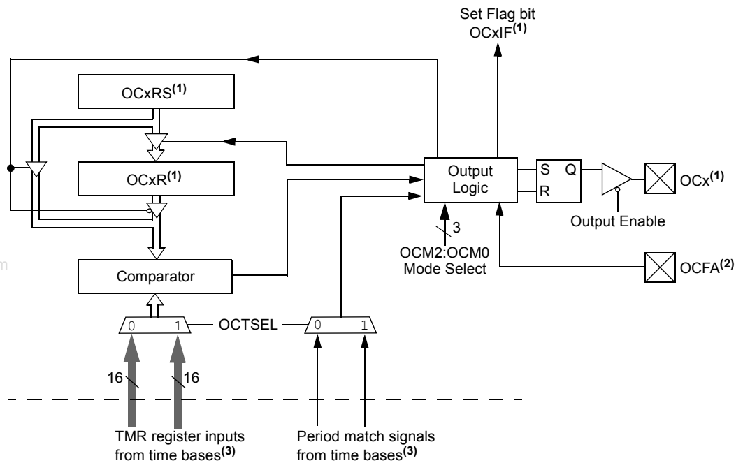
FIGURE 13-1: OUTPUT COMPARE MODULE BLOCK DIAGRAM
