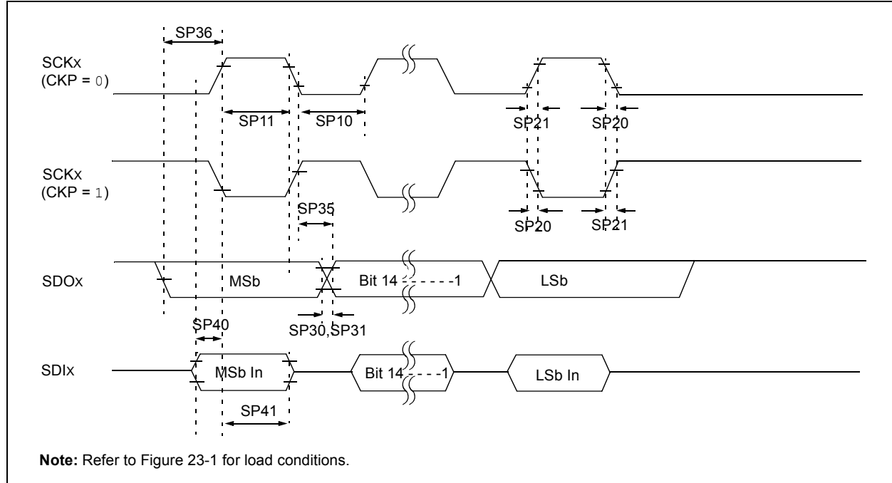
FIGURE 23-15: SPIx MODULE MASTER MODE (CKE = 1) TIMING CHARACTERISTICS www.DataSheet4U.com
