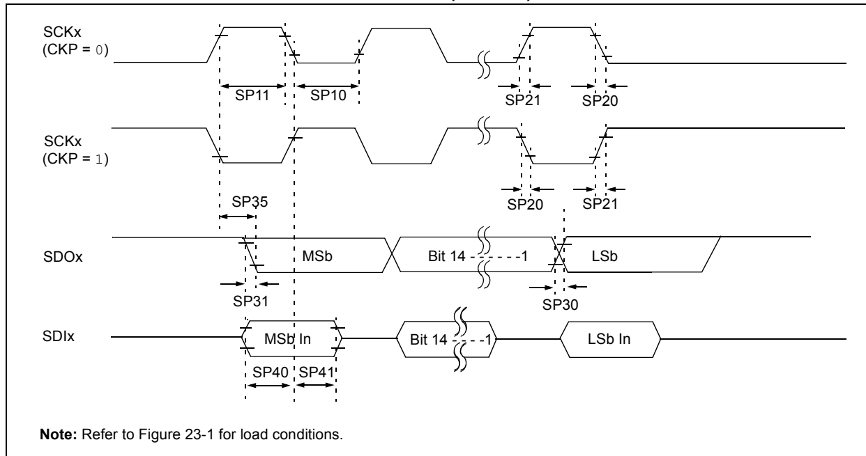
FIGURE 23-14: SPIx MODULE MASTER MODE (CKE = 0) TIMING CHARACTERISTICS www.DataSheet4U.com
