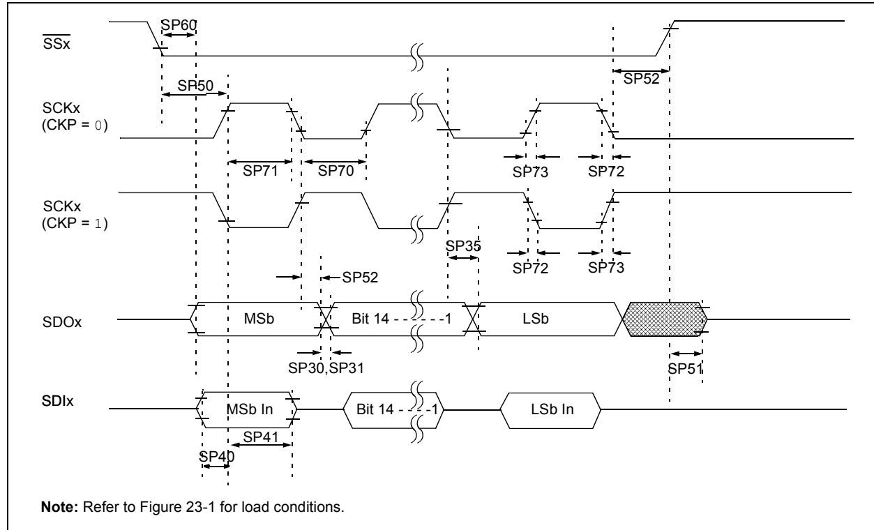
FIGURE 23-17: SPIx MODULE SLAVE MODE (CKE = 1) TIMING CHARACTERISTICS www.DataSheet4U.com
