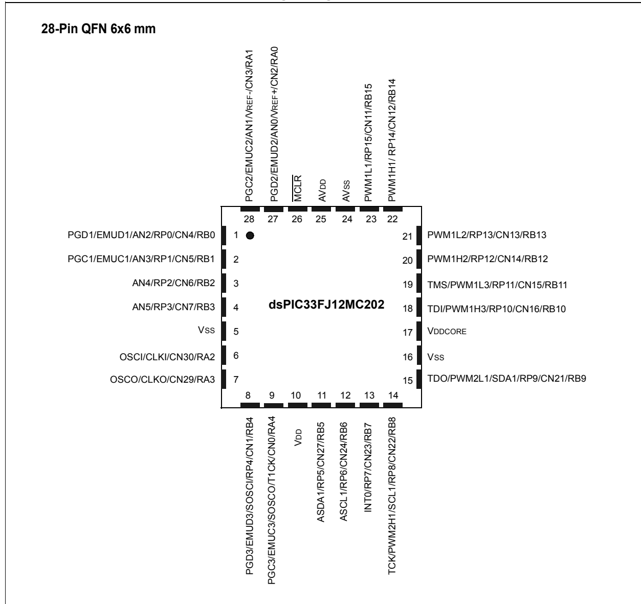
dsPIC33FJ12MC202 28-Pin QFN Package Diagram
