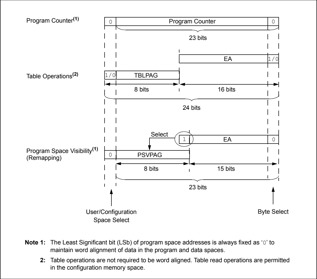
FIGURE 3-7: DATA ACCESS FROM PROGRAM SPACE ADDRESS GENERATION www.DataSheet4U.com
