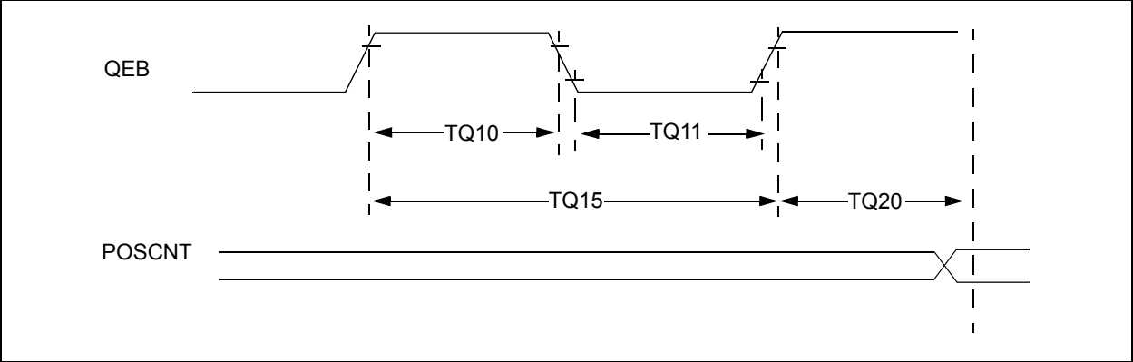
FIGURE 23-6: TIMERQ (QE1 MODULE) EXTERNAL CLOCK TIMING CHARACTERISTICS www.DataSheet4U.com
