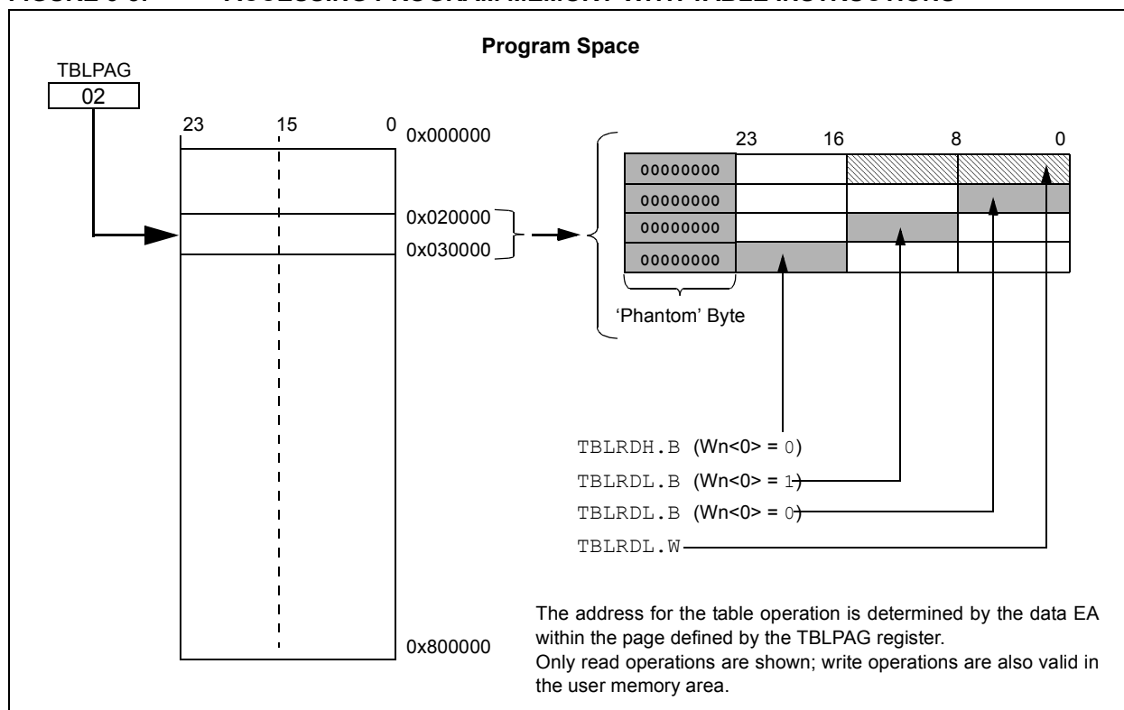
FIGURE 3-8: ACCESSING PROGRAM MEMORY WITH TABLE INSTRUCTIONS
