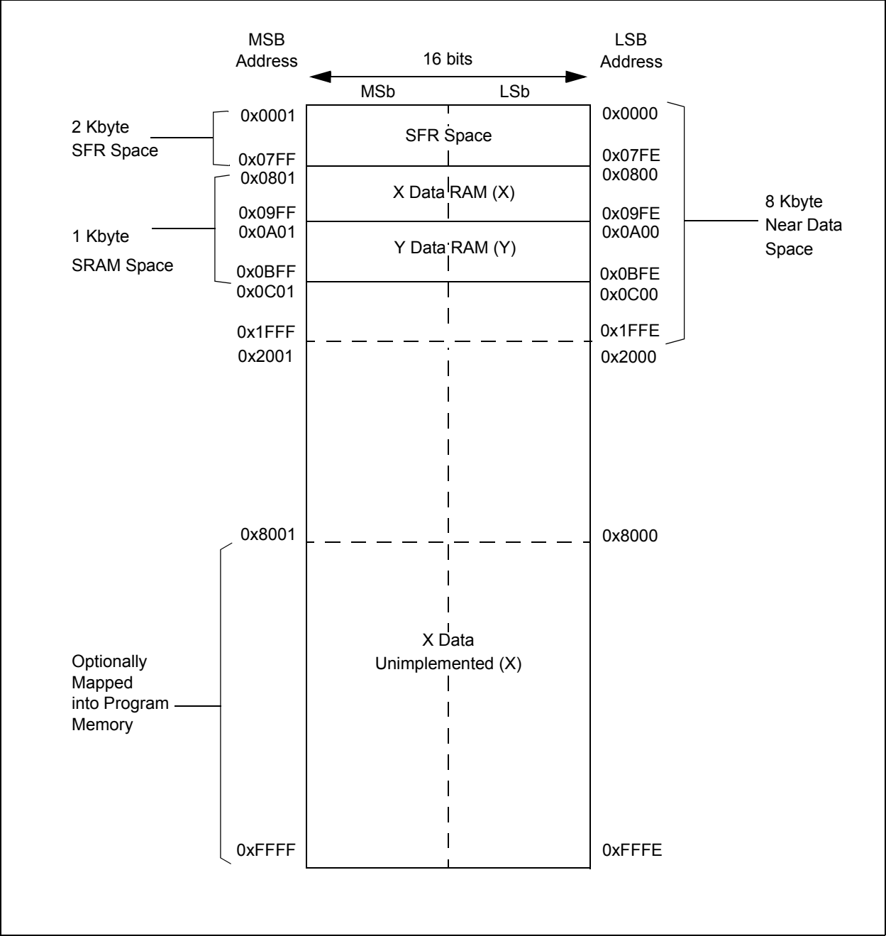
FIGURE 3-3: DATA MEMORY MAP FOR dsPIC33FJ12MC201/202 DEVICES WITH 1 KB RAM www.DataSheet4U.com
