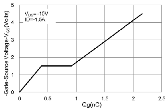
Fig.7 Gate-Charge Characteristics
