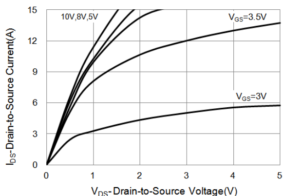
Fig.1 On-Region Characteristics
