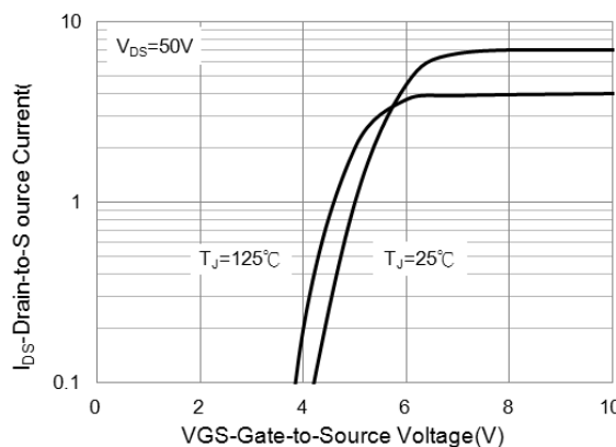
Fig.2 Transfer Characteristics
