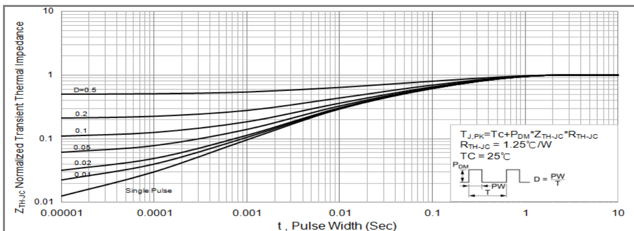
Fig.14 PJP6NA40 Normalized Transient Thermal Impedance vs. Pulse Width
