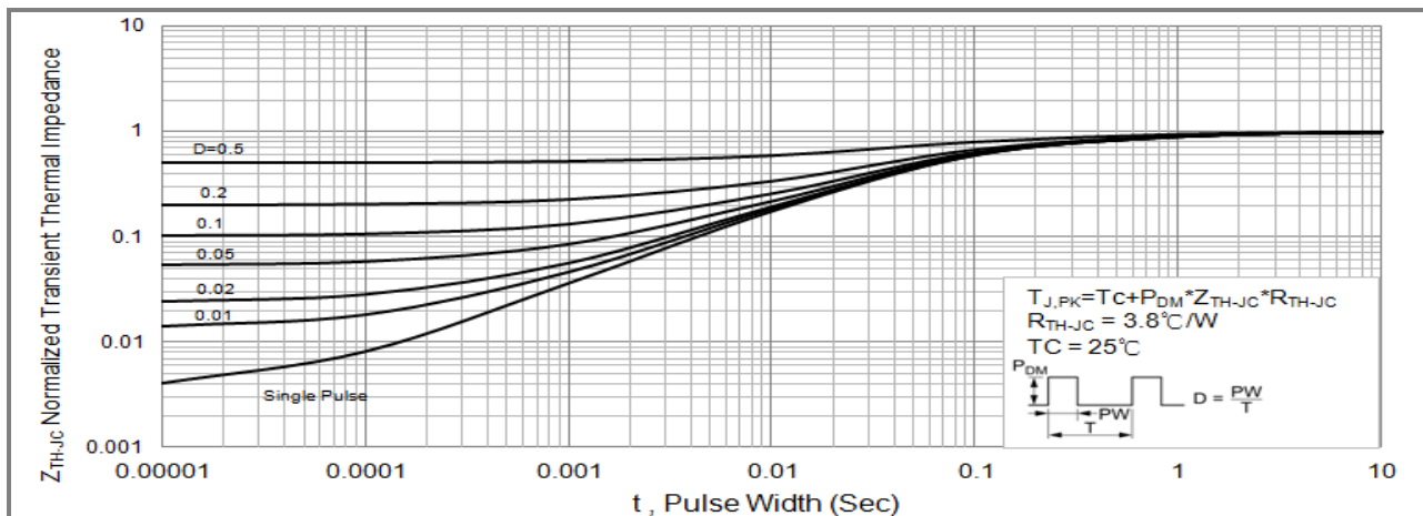
Fig.15 PJF6NA40 Normalized Transient Thermal Impedance vs. Pulse Width
