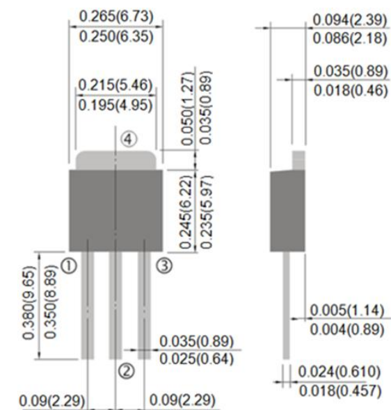
TO-251AA Dimension
